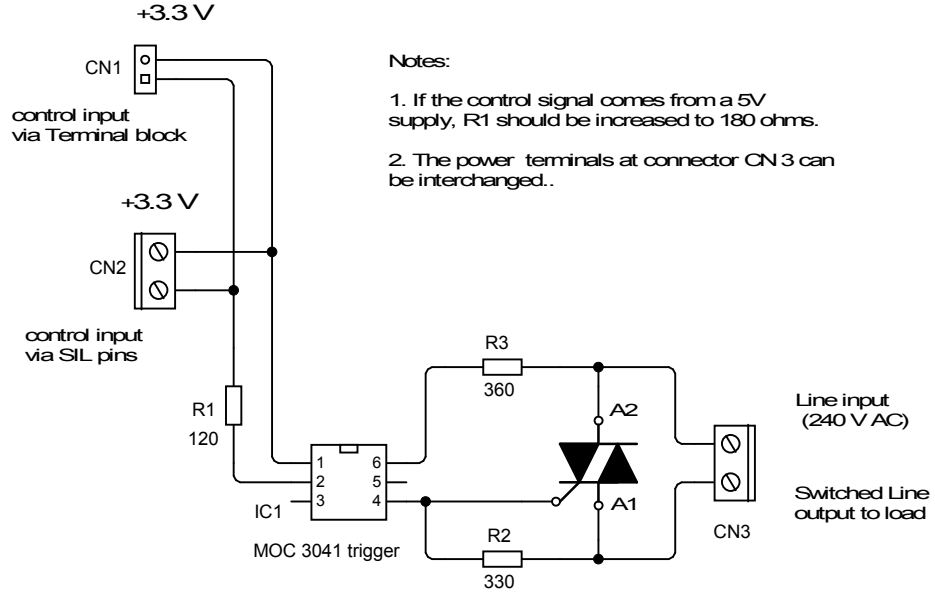
Schematic diagram for the Output PCB
